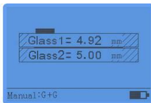
Laminated glass
