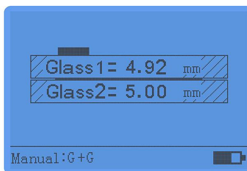
Laminated glass
